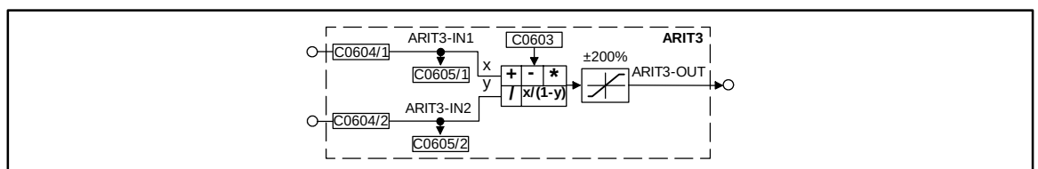
Arithmetics (ARIT3)
