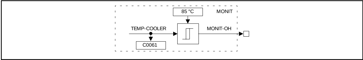
Fig. 7-171 Monitoring of the heat sink temperature, with fixed threshold (OH)
