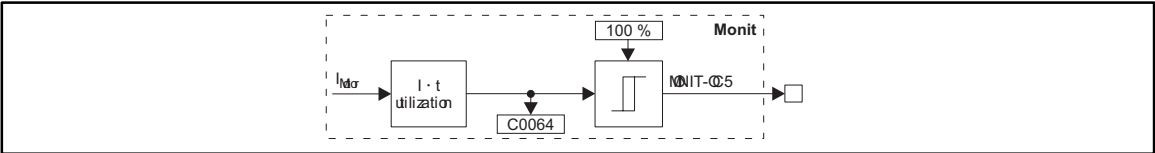
Fig. 7-170 Monitoring of the I x t overload (OC5)
