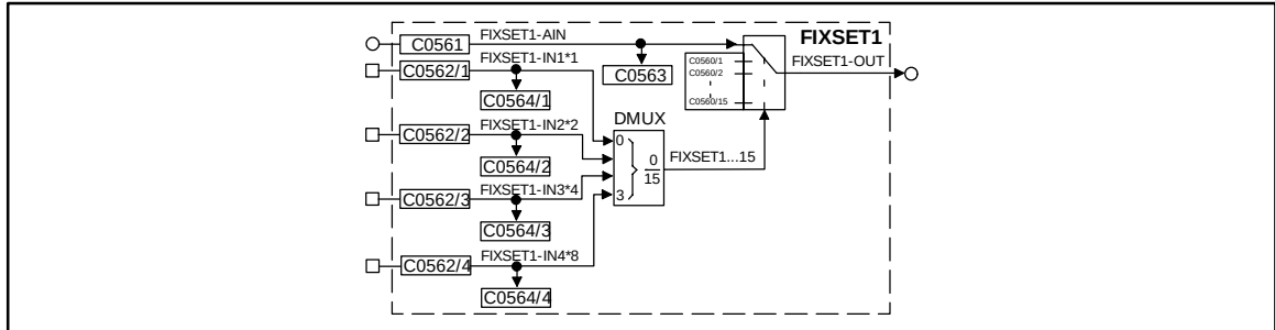
Programming of fixed setpoints (FIXSET1)
