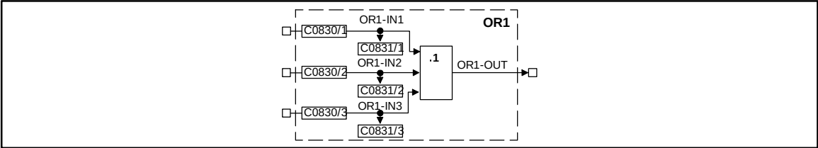
Fig. 7-129 Logic OR (OR1)
