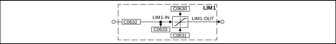
Fig. 7-106 Limitation (LIM1)
