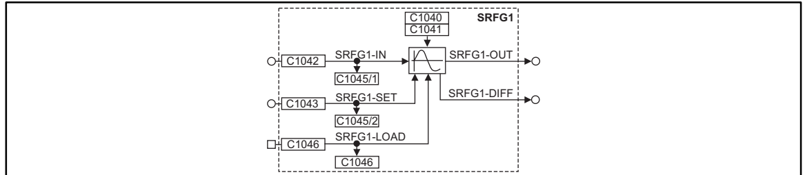
S-ramp function generator (SRFG1)
