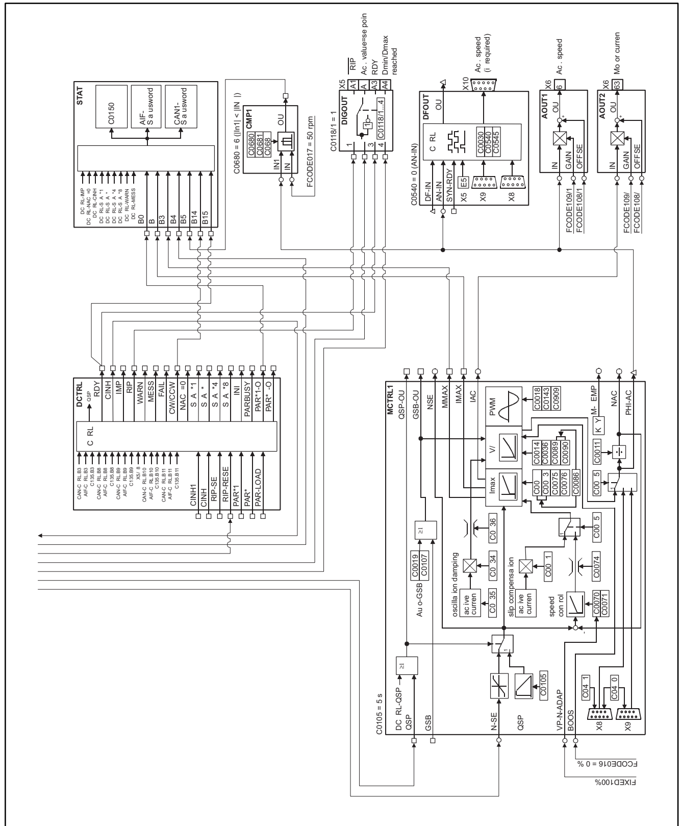
Fig. 16-26 Basic configuration 8000 - dancer position control with external diameter calculator (sheet 2)
