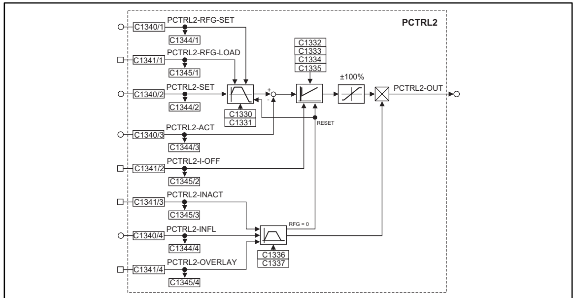
Fig. 7-137 Process controller (PCTRL2)
