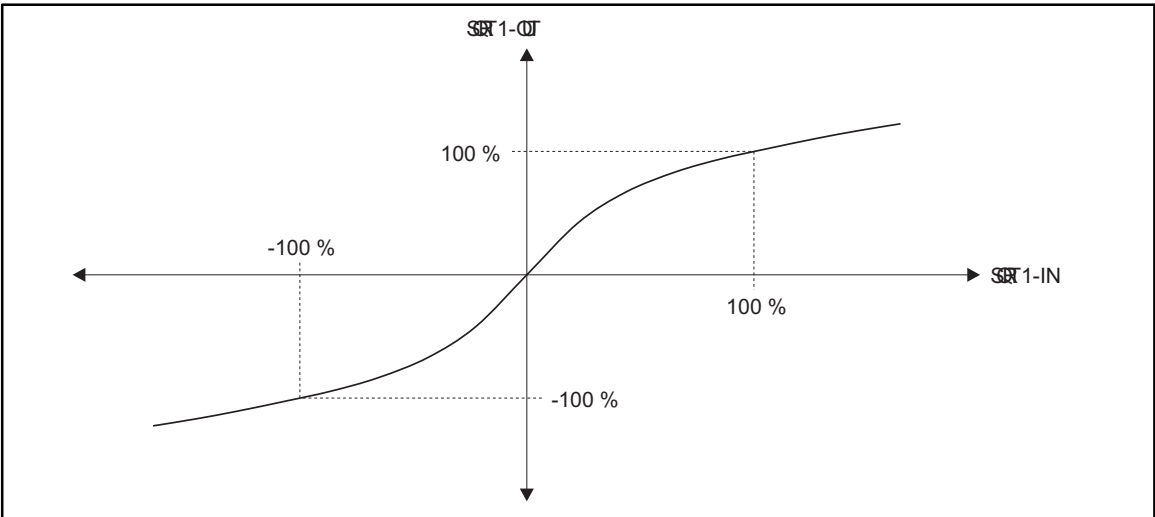
Fig. 7-149 Characteristic of the output signal at SQRT1-OUT to the input signal at SQRT1-IN
