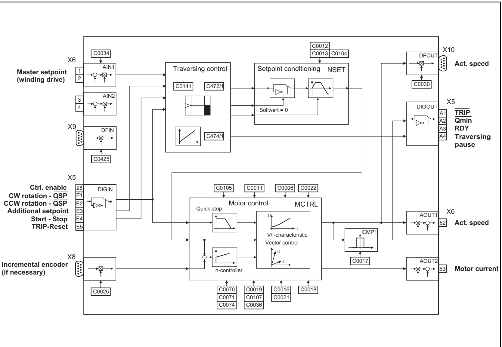
Signal flow for configuration 3000: Traversing control
