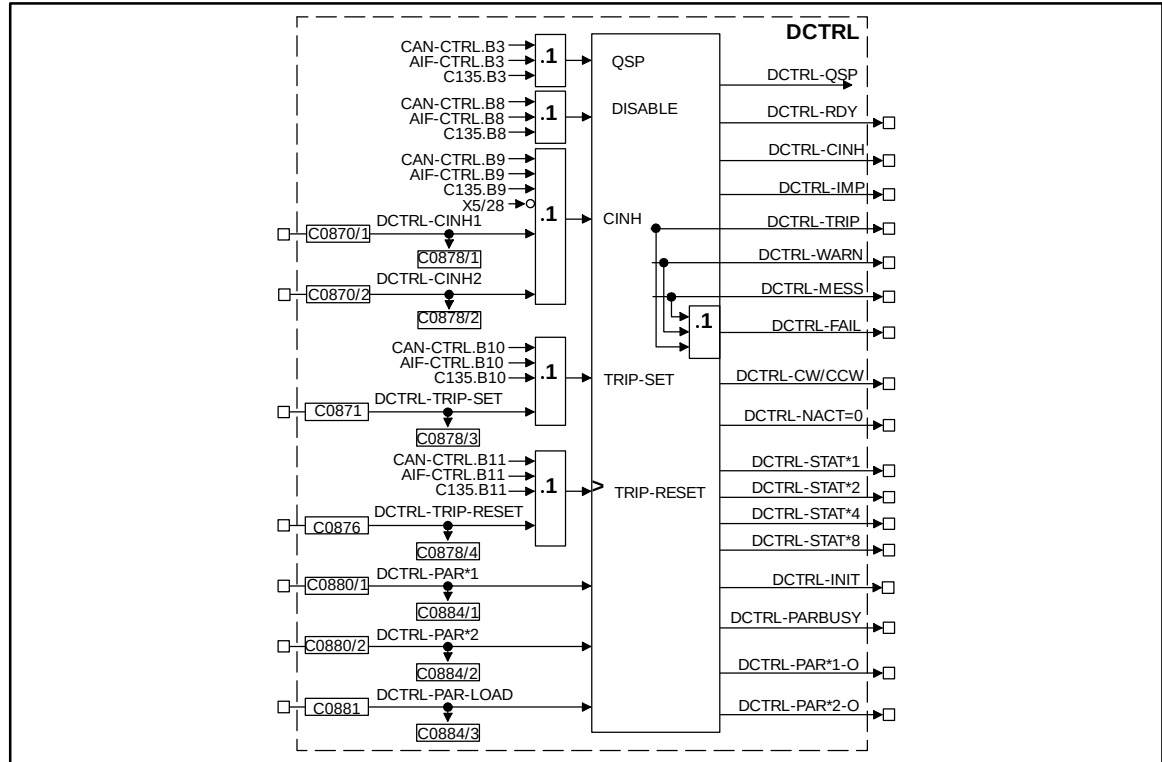
Fig. 7-71 Device control (DCTRL)
