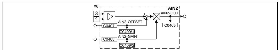
Fig. 7-21 Analog input via terminal X6/3, 4 (AIN2)
