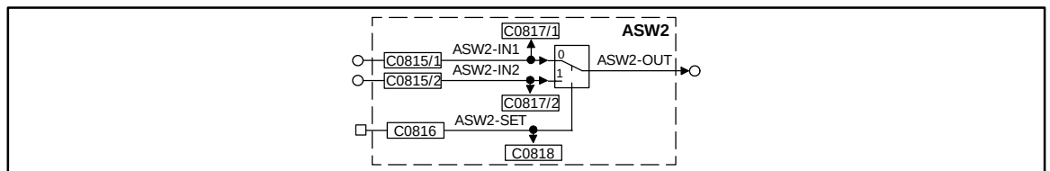
Toggling (ASW2)
