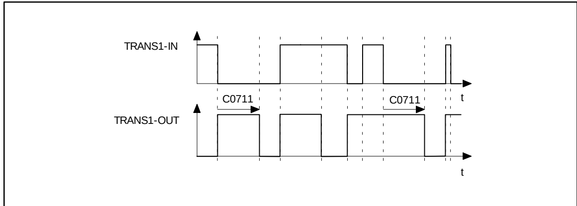
Fig. 7-158 Evaluation of positive and negative edges (TRANS1)
