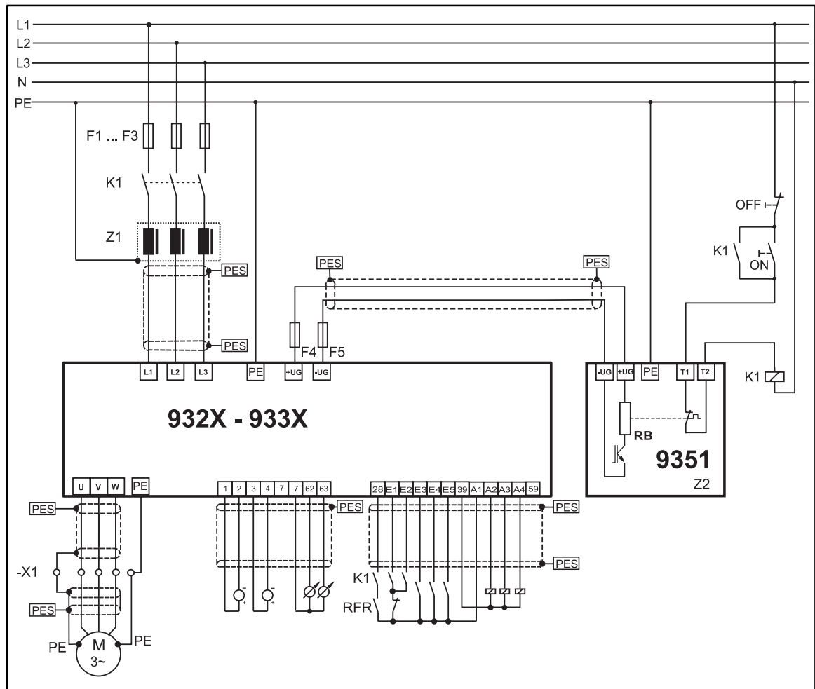
Example of an installation in accordance with the EMC regulations
