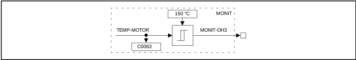
Fig. 7-164 Monitoring of the motor temperature, with fixed threshold (OH3)
