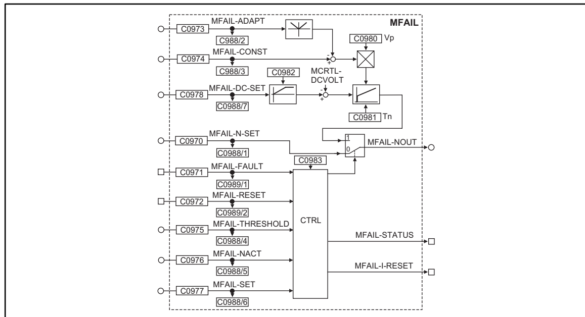
Fig. 7-109 Mains failure control (MFAIL)
